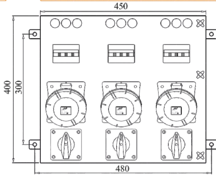
Distribution Box With Interlock 63A Socket-3Nos, 63A 4 Pole MCB-3Nos, 63A Rotary Switch-3Nos & Indicator
