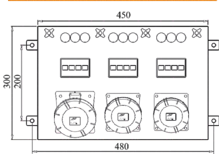
Distribution Box With 63A, 32A & 16A Sockets, 63A, 32A & 16A 4 Pole MCB, & Indicator
