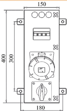
Distribution Box With Interlock 63A Socket, 63A 4 Pole MCB, 63A Rotary Switch & Indicator
