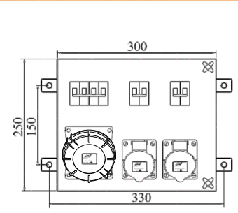
Distribution Box With 32A, 16A Sockets, 32A & 16A MCB, & Indicator
