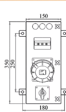
Distribution Box With Interlock 32A Socket, 32A 4 Pole MCB, 32A Rotary Switch & Indicator
