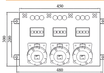
Distribution Box With 63A Sockets-3Nos, 63A 4 Pole MCB-3Nos, & Indicator
