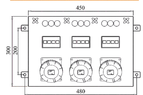
Distribution Box With 32A Sockets-3Nos, 32A 4 Pole MCB-3Nos, & Indicator
